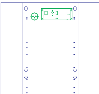
MX4428 6A PSU Brick Mounting
