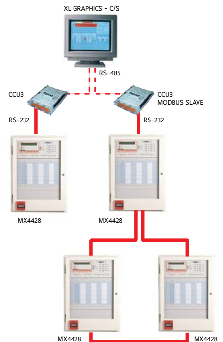
Two methods of connecting CCU3/C-MXMB to VIGILANT MX4428 CIE
