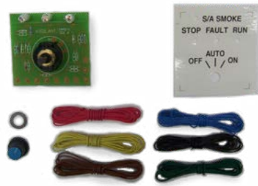
KTO113 Kit, AS 1668 Control Module Type 3
