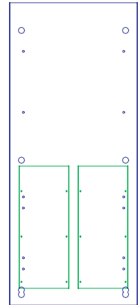
F3200 Card Frame Mounting
