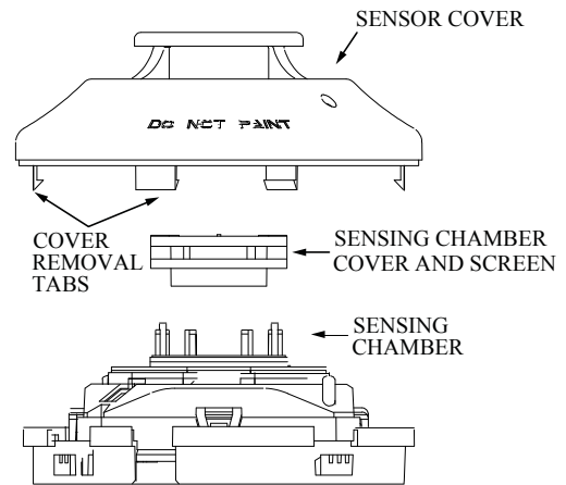
FIGURE 4. SENSOR ASSEMBLY:
