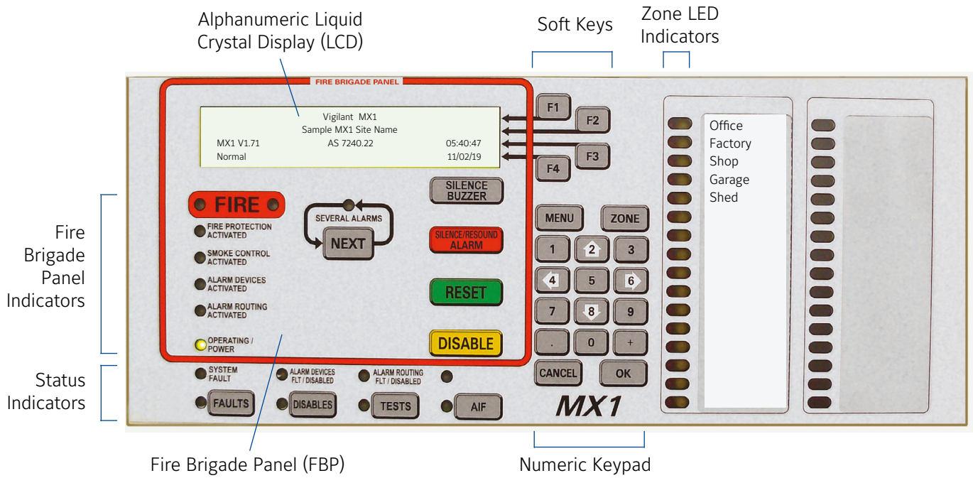
Fig 1-1 Operator Interface
