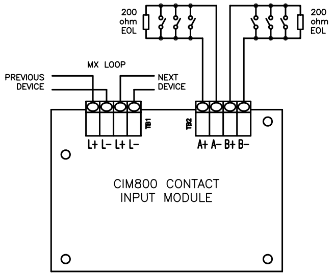
NORMALLY OPEN
