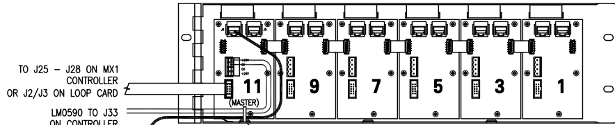
EXAMPLE 2 DOOR WITH 2 CONTROL BOARDS FITTED
