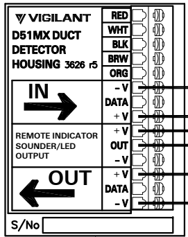
D51MX DUCT SAMPLING UNIT
