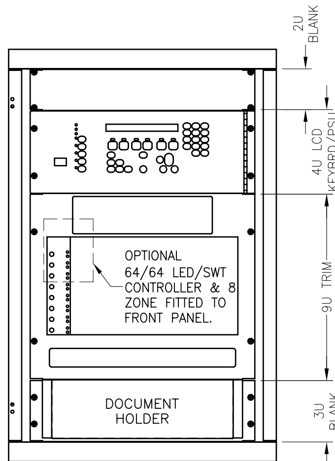
FRONT VIEW NO OUTER DOOR
