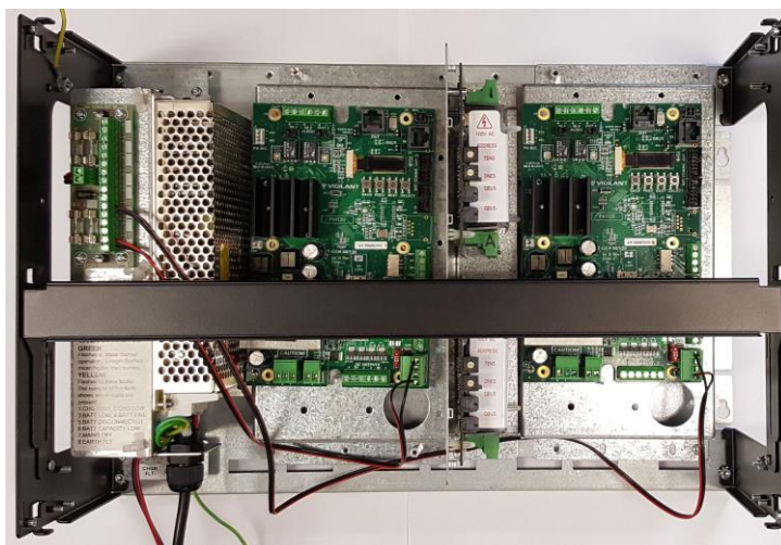
Figure 7 PDI Bay with 2 x T-Gens, Splitter & 5A PSU
