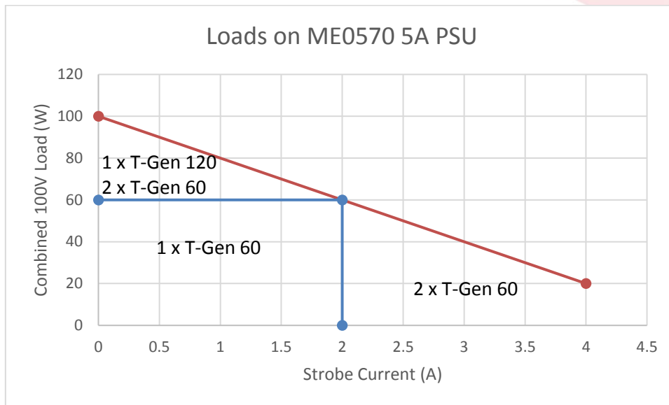
Figure 8 Supported T-Gen2 Loads on 5A ME0470
