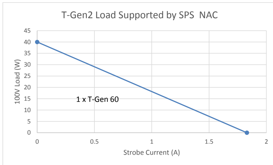
Figure 9 T-Gen2 Load Supported by SPS NAC/AUX Output
