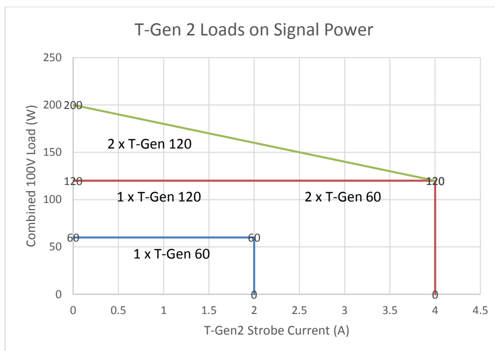
Figure 6 Supported T-Gen2 Load on Signal Power
