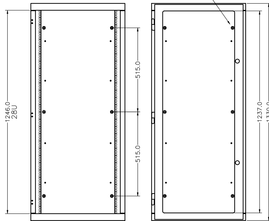
INSIDE VIEW 28U CABINET
