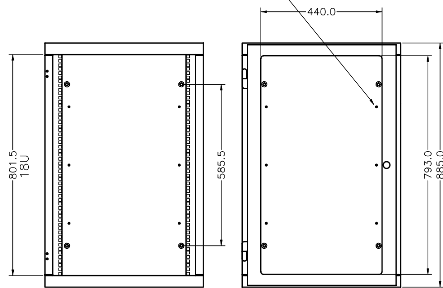
INSIDE VIEW 18U CABINET
