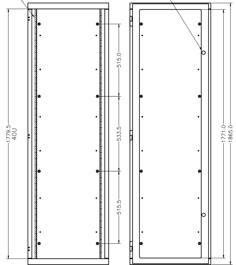
INSIDE VIEW 40U CABINET
